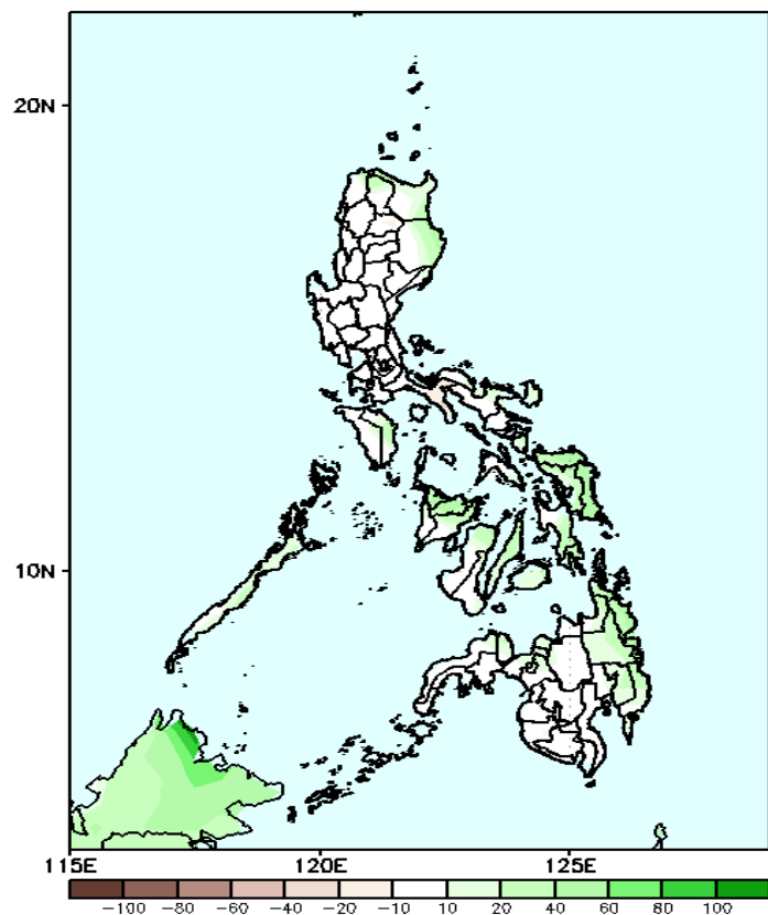
GEFS Week-2 Precip Anomaly Valid: 20250110 - 20250116
