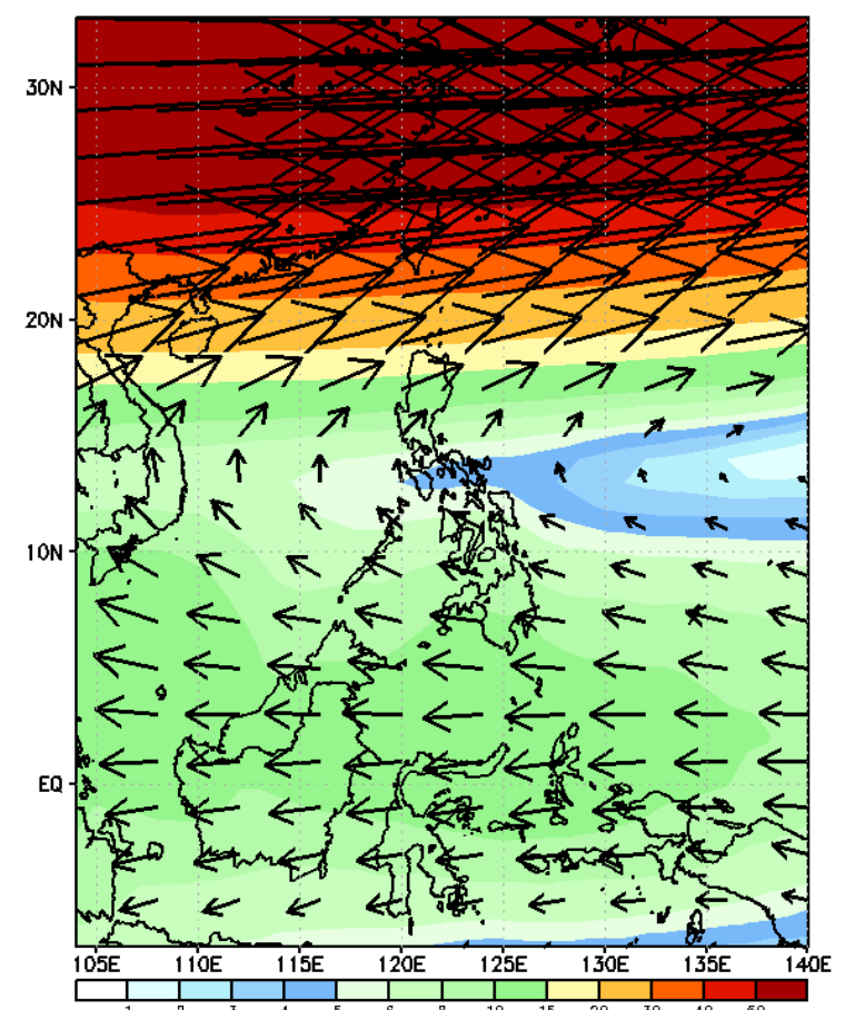
GEFS Week-2 200-hPa Wind Total Valid: 20250110 - 20250116
