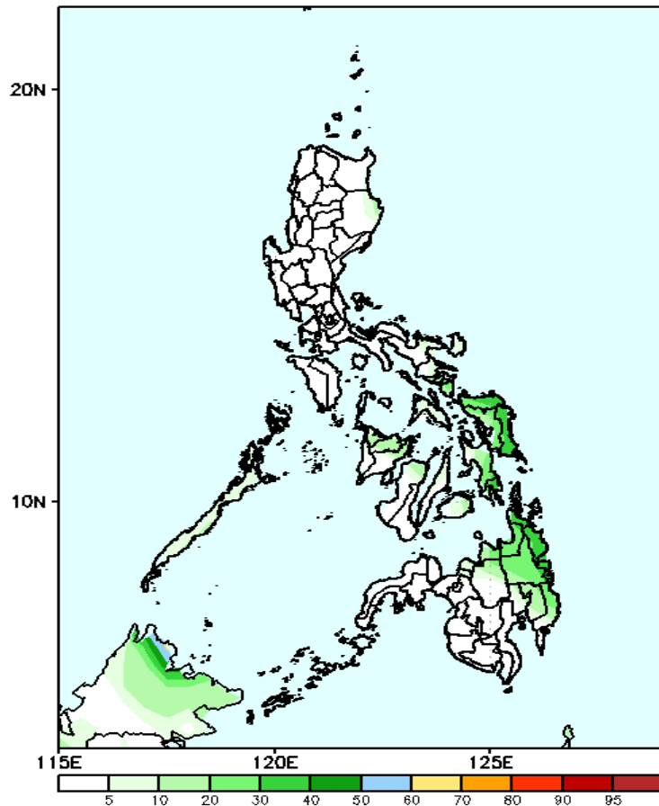
GEFS Week-2 Exceedance Prob. > 150mm Valid: 20250110 - 20250116
