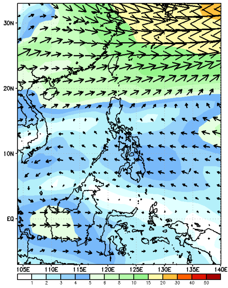
GEFS Week-1 700-hPa Wind Total Valid: 20250103 - 20250109
