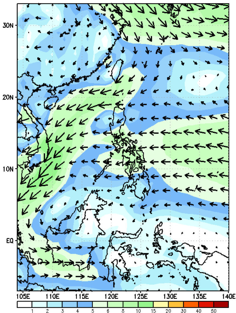
GEFS Week-1 850-hPa Wind Total Valid: 20250103 - 20250109
