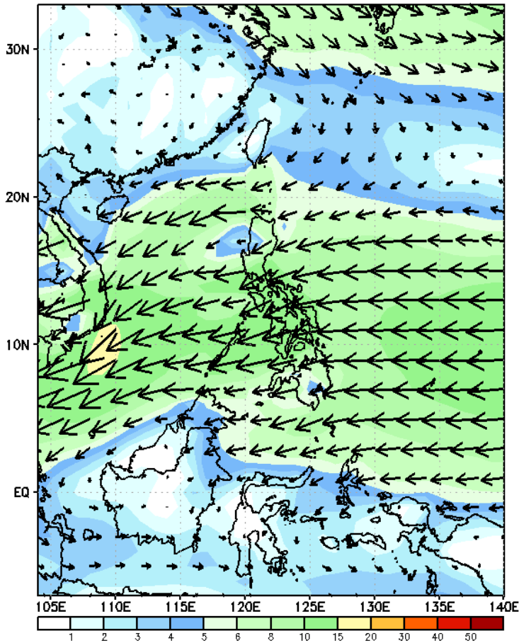
GEFS Week-2 850-hPa Wind Total Valid: 20250110 - 20250116
