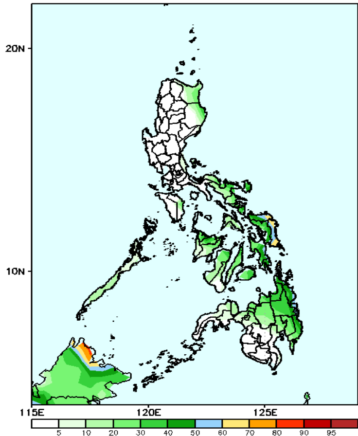
GEFS Week-2 Exceedance Prob. > 100mm Valid: 20250110 - 20250116
