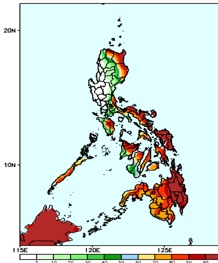
GEFS Week-2 Exceedance Prob. > 25mm Valid: 20250110 - 20250116
