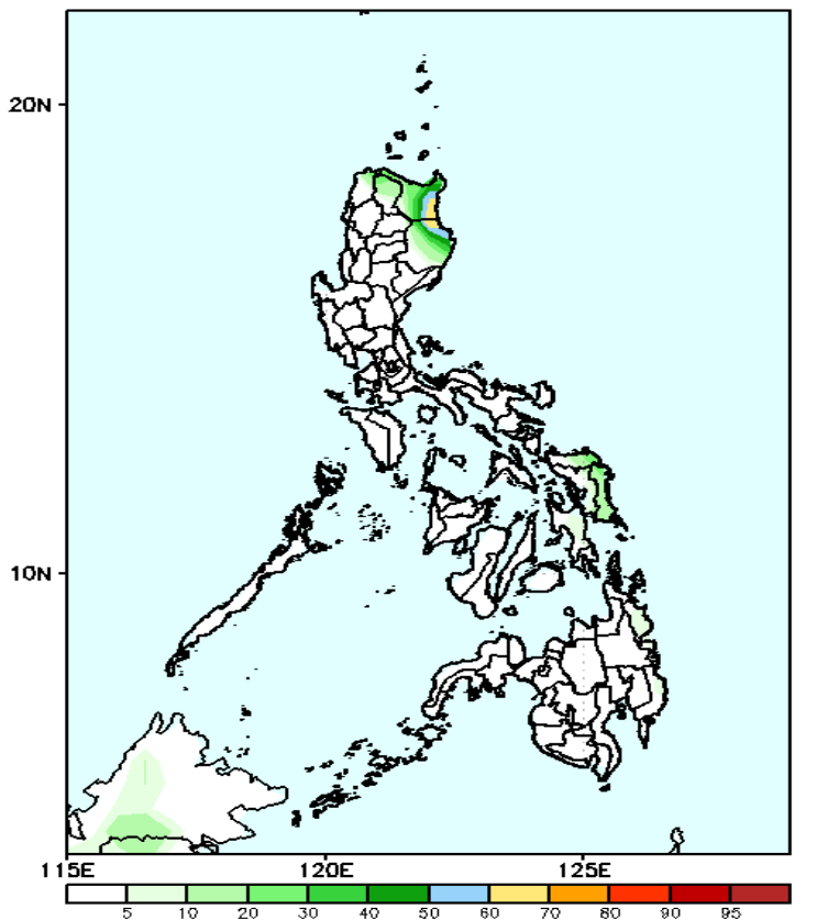
GEFS Week-1 Exceedance Prob. > 150mm Valid: 20250103 - 20250109
