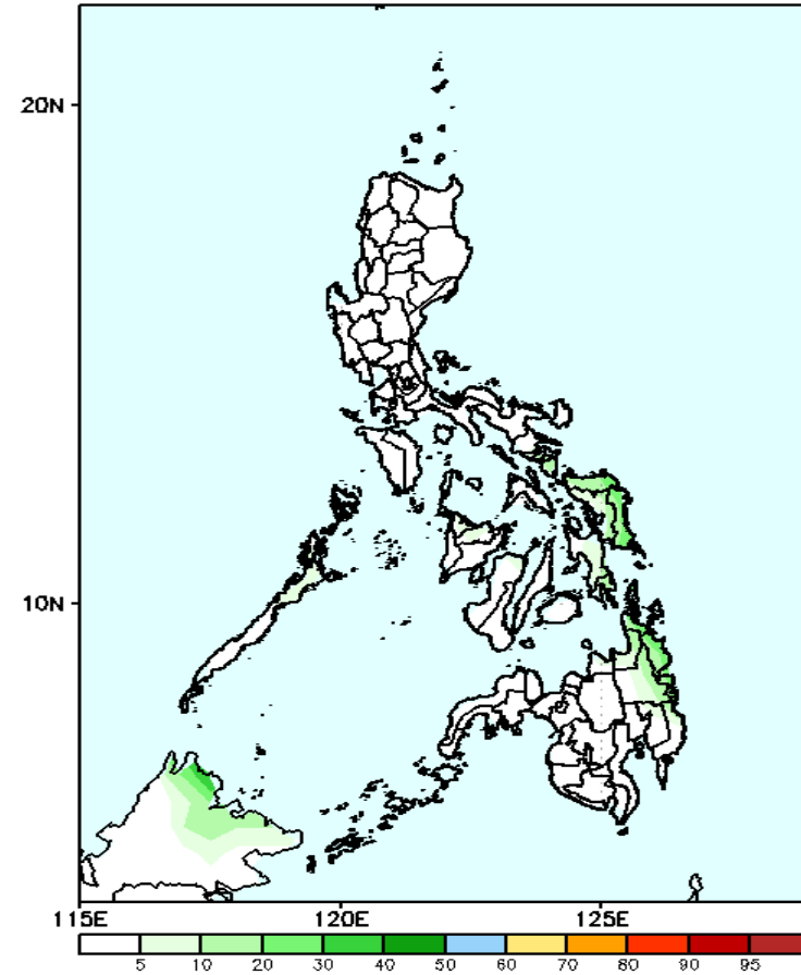
GEFS Week-2 Exceedance Prob. > 200mm Valid: 20250110 - 20250116
