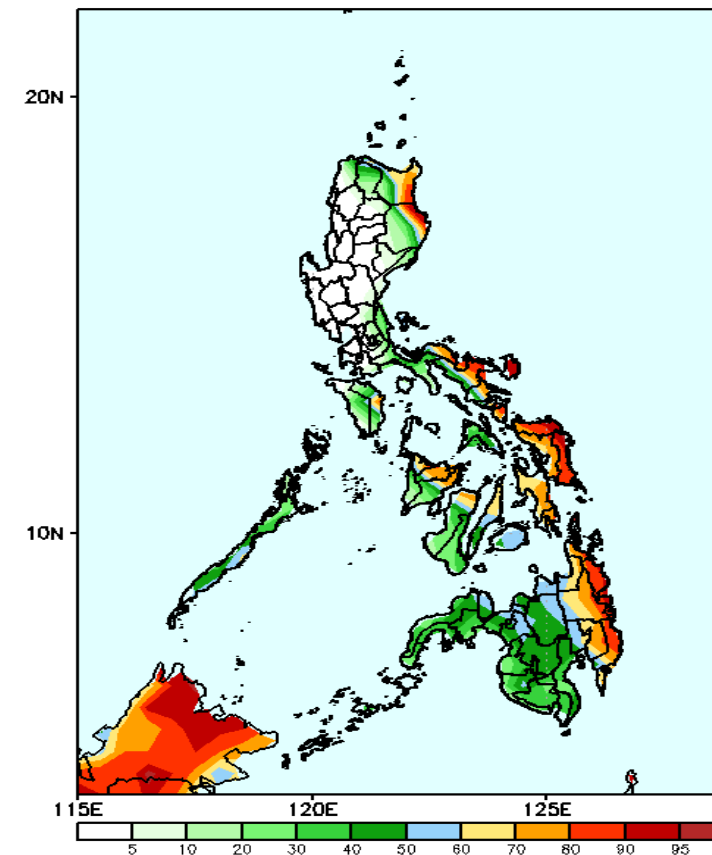
GEFS Week-2 Exceedance Prob. > 50mm Valid: 20250110 - 20250116
