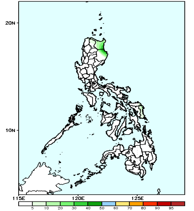
GEFS Week-1 Exceedance Prob. > 200mm Valid: 20250103 - 20250109
