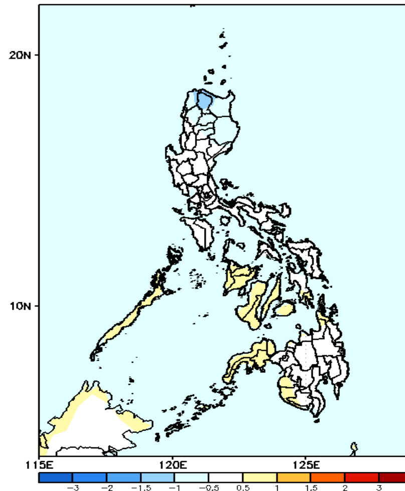
GEFS Week-2 T2m Anomaly Valid: 20250110 - 20250116
