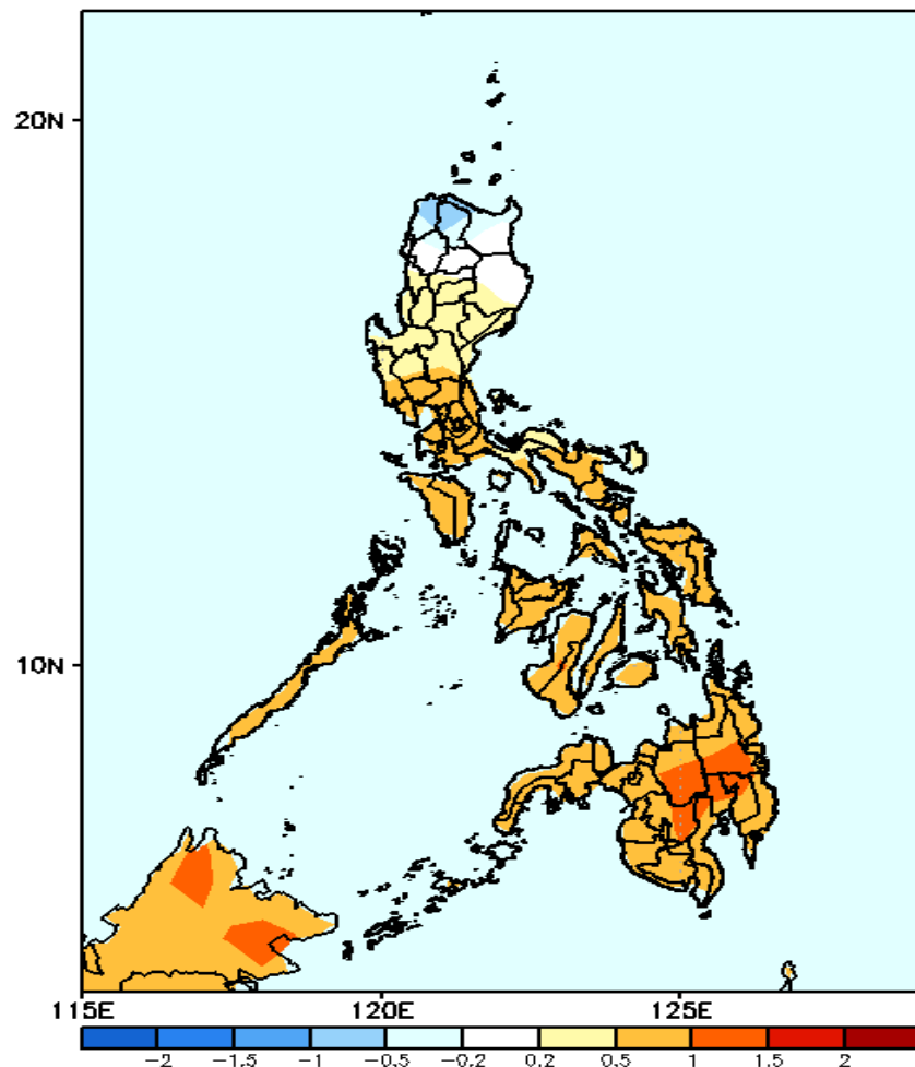
GEFS Week-1 T2m Anomaly Valid: 20250103 - 20250109
