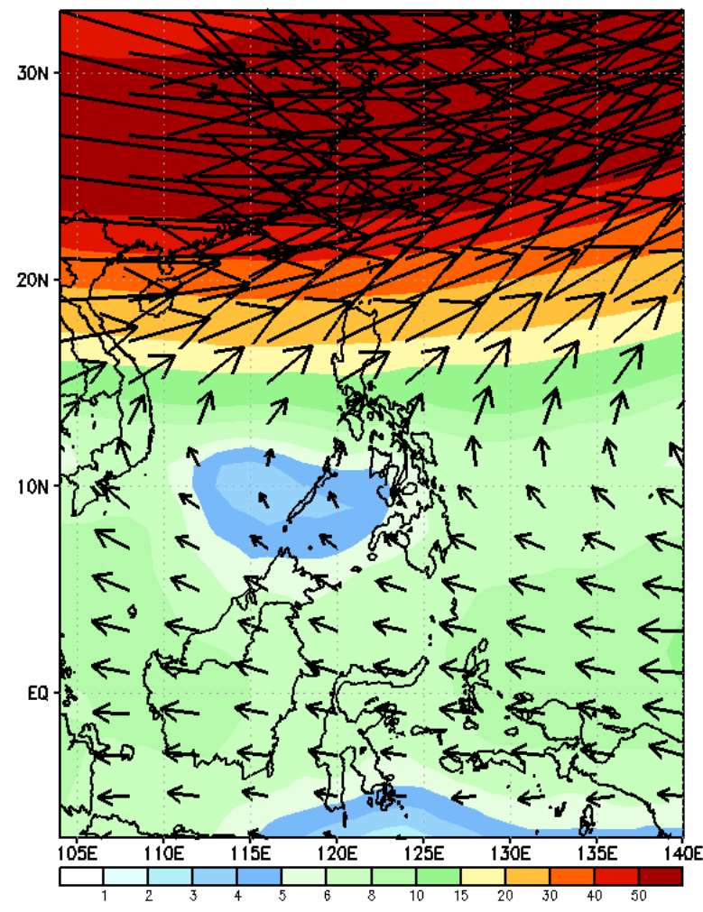
GEFS Week-1 200-hPa Wind Total Valid: 20250103 - 20250109
