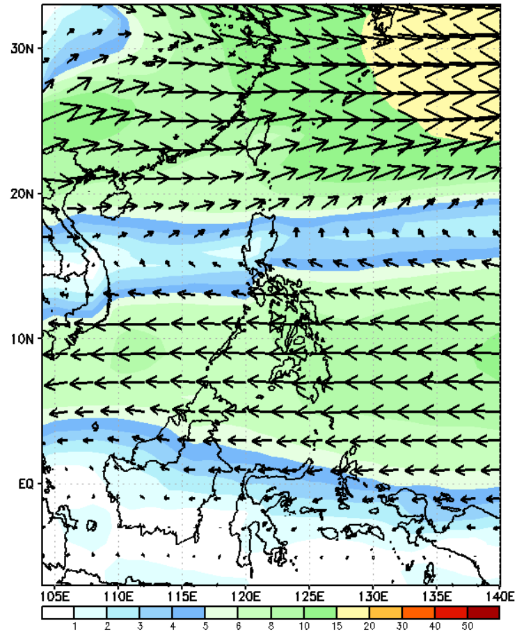
GEFS Week-2 700-hPa Wind Total Valid: 20250110 - 20250116
