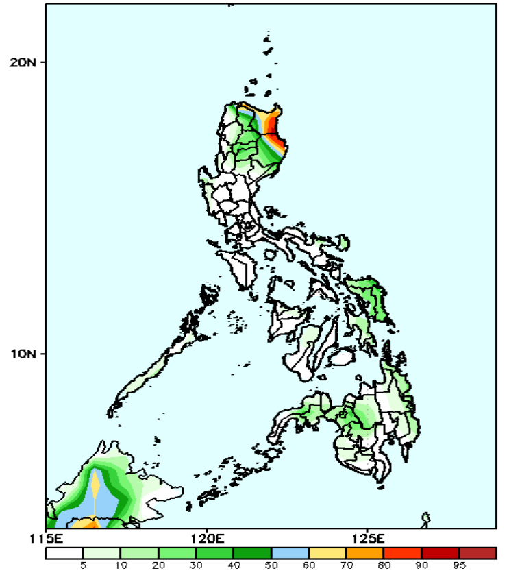
GEFS Week-1 Exceedance Prob. > 100mm Valid: 20250103 - 20250109
